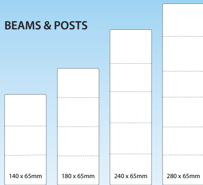
Beams: Finger jointed laminated GL8
