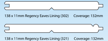
138 x 11mm Regency Eaves Lining (321) Coverage: 132mm
