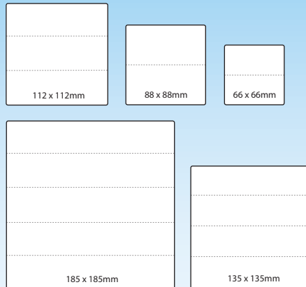
Posts: Finger joint laminated GL8
