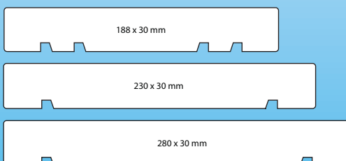
Weatherboard Stop
